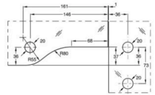
Cut Out for DPF-40
