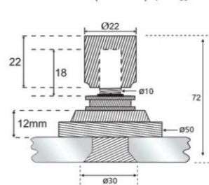
DSP-FB-FL Fix Routel (Flat Head)
