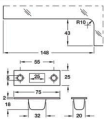
Cut Out for DPL-10
