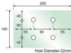
DSP-200 Splice Plate 200mm
