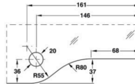
Cut Out for DPF-30
