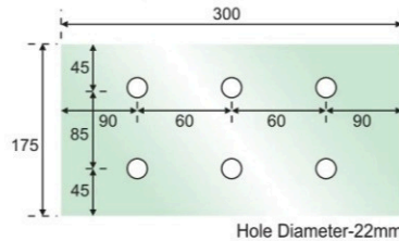
DSP-300 Splice Plate 300mm
