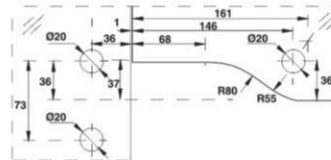
Cut Out for DPF-41 (L) & DPF-41 (R)
