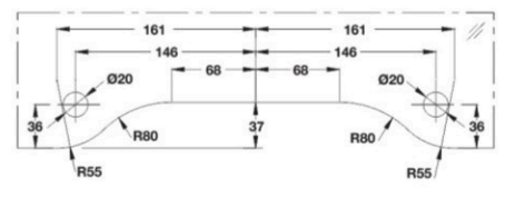
Cut Out for DPF-61
