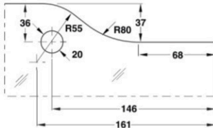
Cut Out for DPF-10
