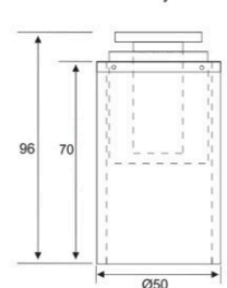
DSA-01 Iron Assembly
