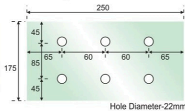
DSP-250 Splice Plate 250mm
