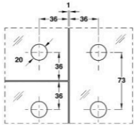
Cut Out for DPF-620
