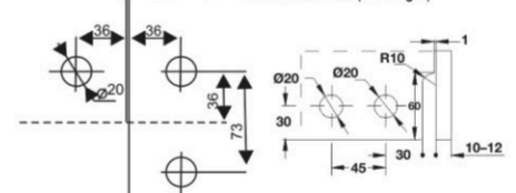
Cut Out for DPF-610 (L/R)
