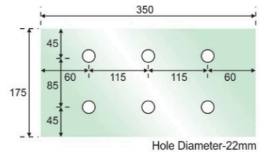
DSP-350 Splice Plate 350mm
