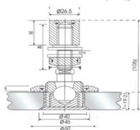
DSP-FB-36CS Articulated Routel with Counter Sunk Hole
