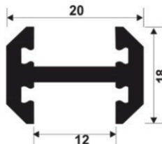
DGP-114 Glass Edge Profile for Partition (Black Matt)
