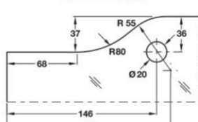
Cut Out for DPL-2A
