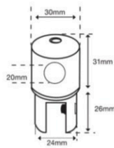
DKH-5 (Brass) Rod to Rod T Connector (Dia 19mm)
