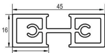
DGP-105 Divider Profile
