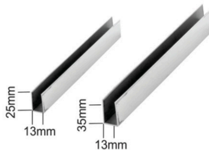
DGPL-2 'U' Channel (For Fixed Glass) Finish: CP/ SS Available in 3.4 Mtr., Thickness: 1.5mm
