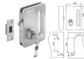
DSDL-13A+13C Sliding Door Lock with Strike Plate
