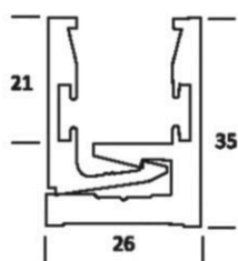
Specification Material : Aluminium For 10 to 12 mm Glass Size : 3, 4 & 5 mtr.
