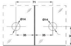
Cut Out for DPF-630
