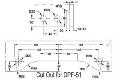
DPF-51 Double Over Panel Patch with Fin
