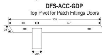
Cut Out for DFS-ACC-GDP
