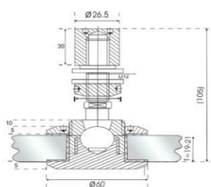
DSP-AFB-36FL Articulated Route
