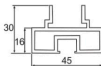
DPTS-106 Top and Bottom Channel
