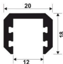
DGP-113 Glass Edge Profile (Black Matt)
