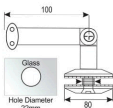
DCF-1 Wall to Glass Connector
