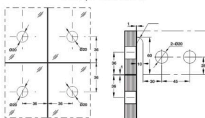
Cut Out for DPF-620 (F)
