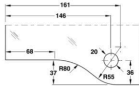
Cut Out for DPF-20
