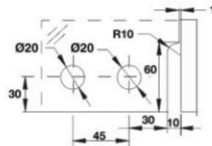
Cut Out for DPF-41 (L) & DPF-41 (R)
