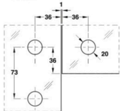
Cut Out for DPF-610
