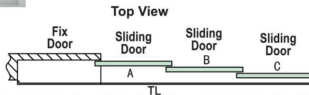
DPSS-100 (Soft Close) Telescopic Sliding System (3 Door)
