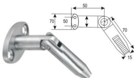
DCF-3 Wall to Rod Connector
