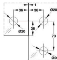
Cut Out for DPF-610 ST
